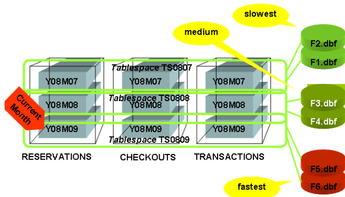
Figure 6 Tablespace Design
